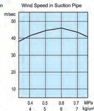
■ Performance Chart (SC60-50S)
