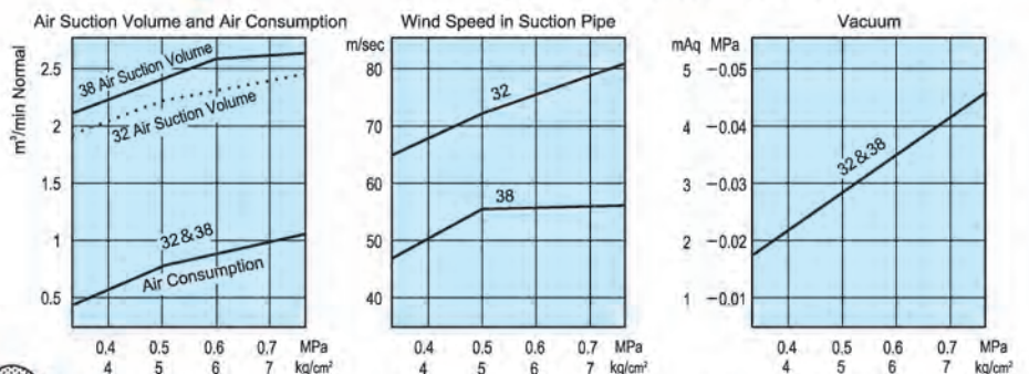
Performance Chart (SC60-32S, SC60-38S, SC200-32D, SC200-38D)
